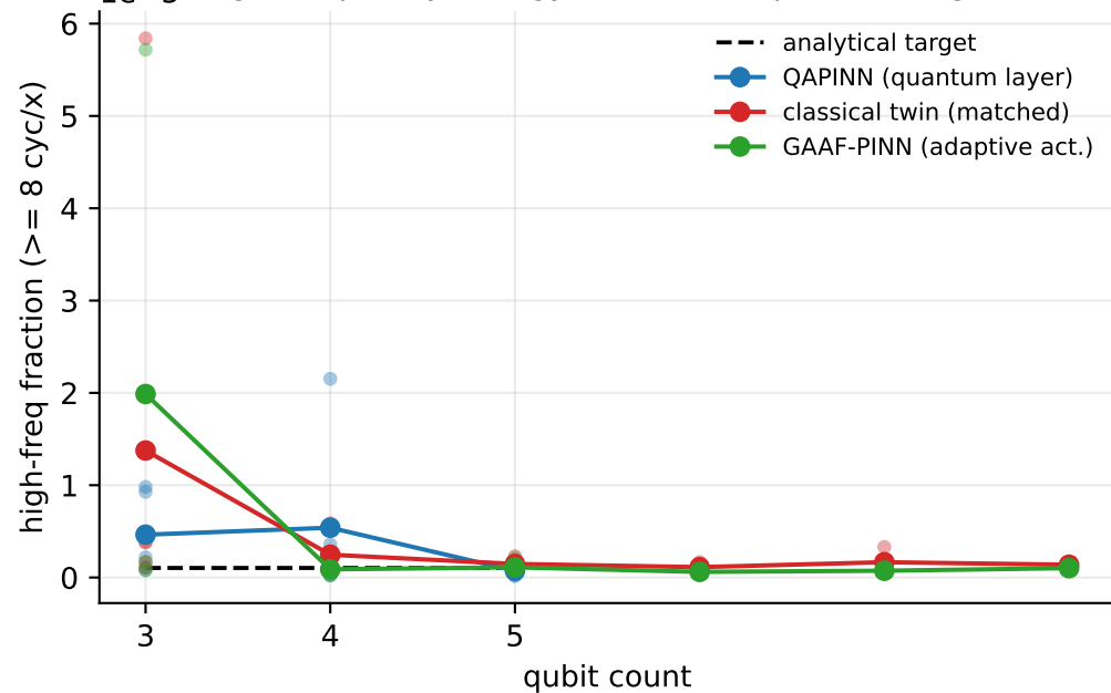
High-frequency energy fraction vs qubits - burgers
