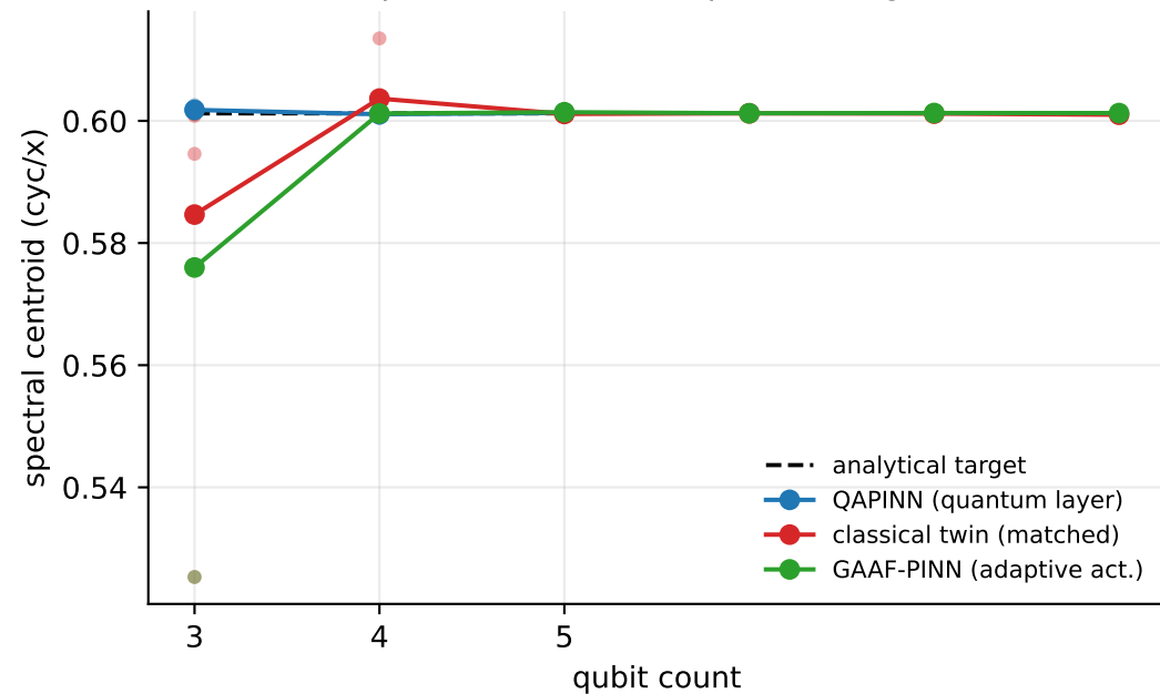
Spectral centroid vs qubits - burgers
